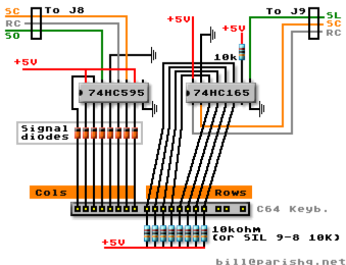
C64 Keyboard connection to MBHP v2 http://ucapps.de
