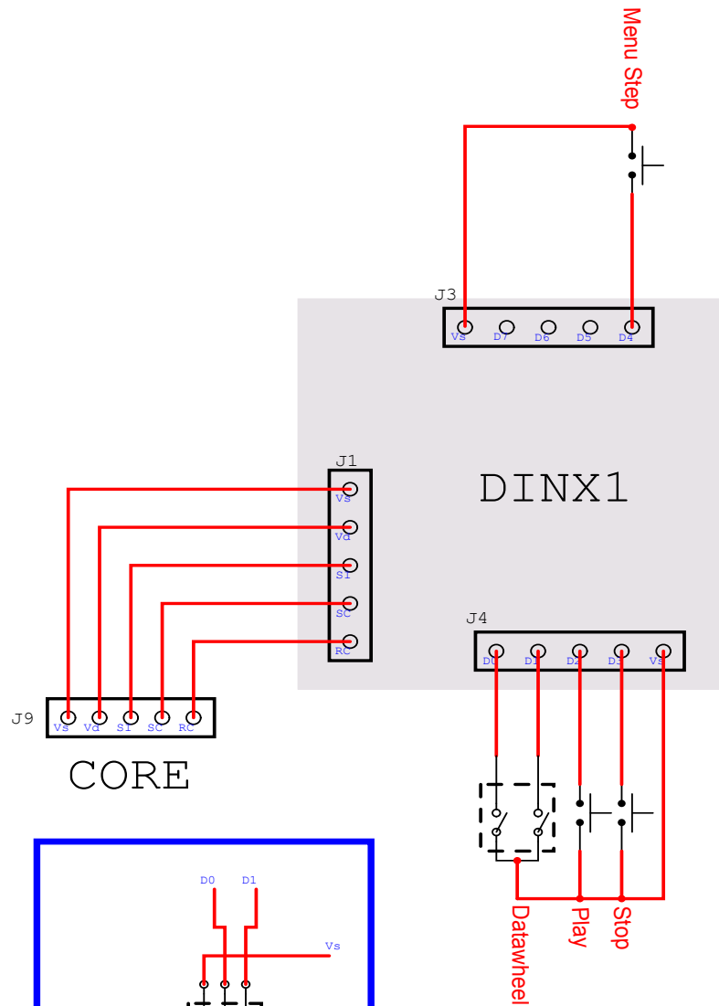
MIDIbox Hardware Platform Visual Metronome DINx1 Button Assignments
