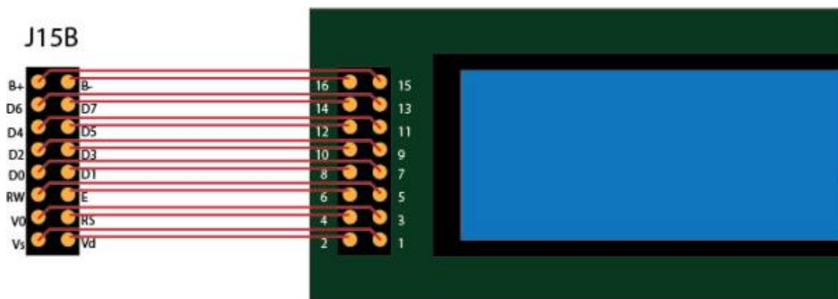
Typical CLCD Pinout Connection
