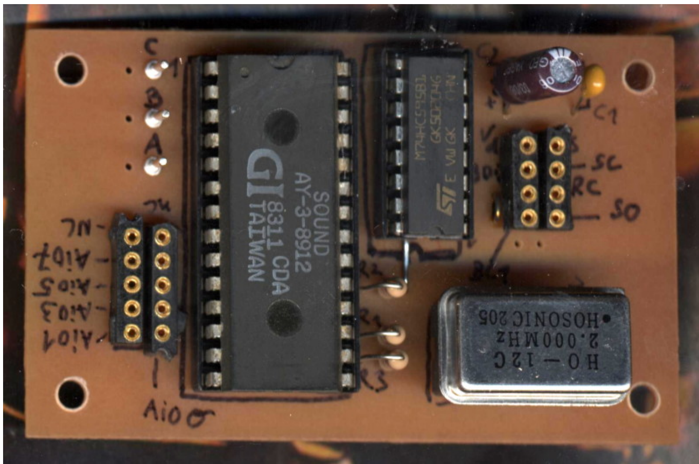
[AY 3 8912 Board]
