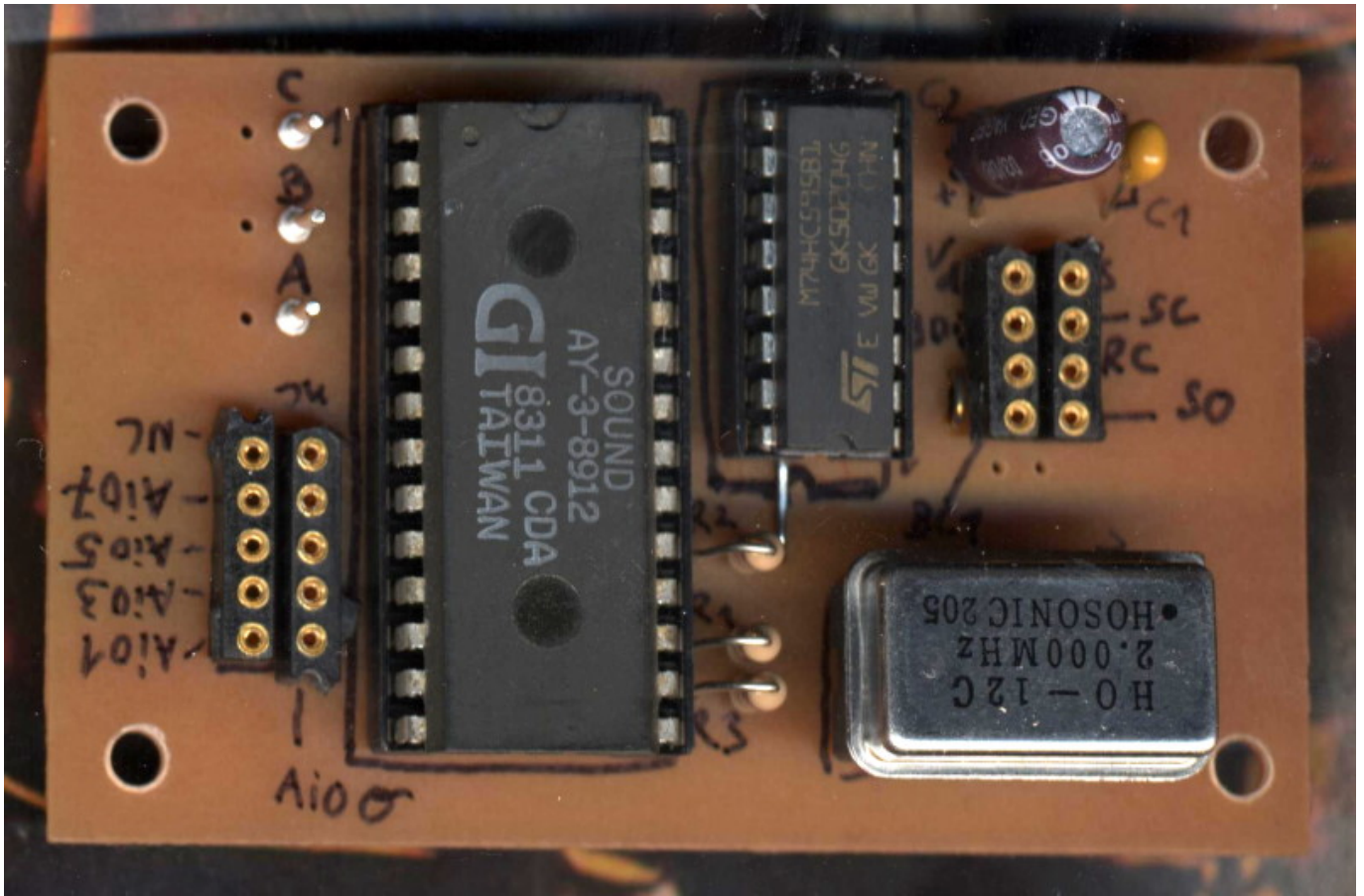
[AY 3 8912 Board]
