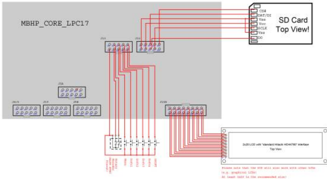
Wiring Diagram for MIDIbox NG SCS © J. T. Kwan 2013-01-02
