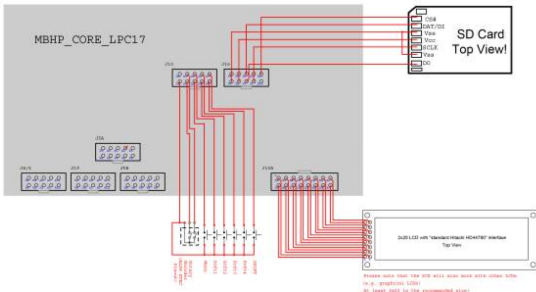
Wiring Diagram for Arduino NOD SCS © T. Kluen 2013-01-02
