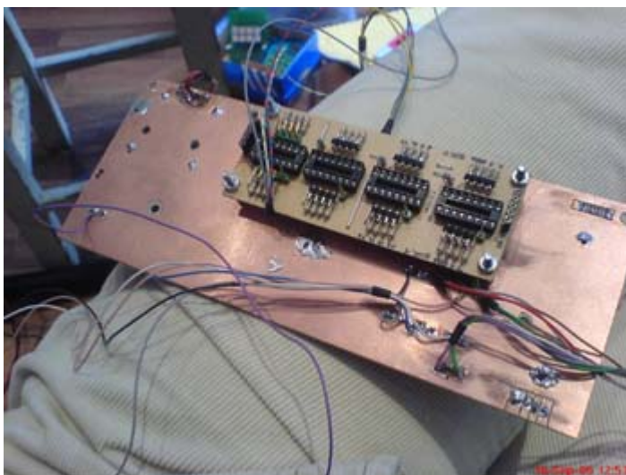
A DIN X4 is piggybacked to each board with M3 screws and spacers.
